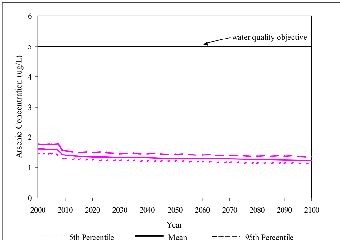
FIGURE 6.1-3 PREDICTED ARSENIC LEVELS – NORTH YELLOWKNIFE BAY WATER
